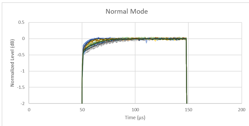
1. Measured with a 500 kHz IF bandwidth, no averaging. With 100 \mu s pulse width setting. 50 \mu s/div.
