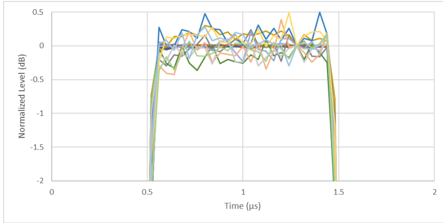
2. Measured with a 15 MHz IF bandwidth, averaging factor of 16 (Average Type = Point). With 1 \mu s pulse width setting. 0.5 \mu s/div. S960250B software is required. (Minimum pulse width with S960240B is 50 \mu s.)
